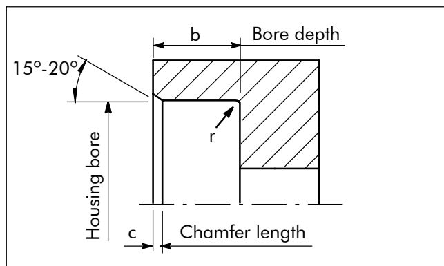
Figure 9 Housing design
