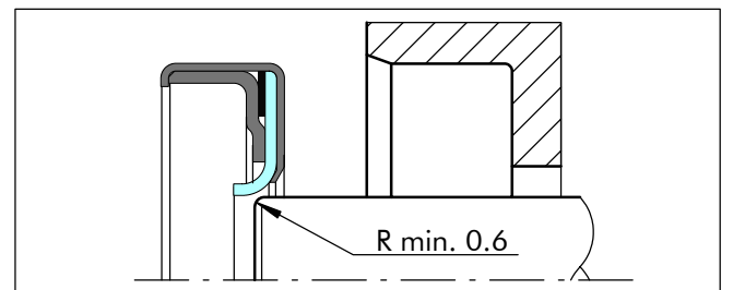
Figure 10 Installation of the sealing lip with the back to the shaft for pressurised application
