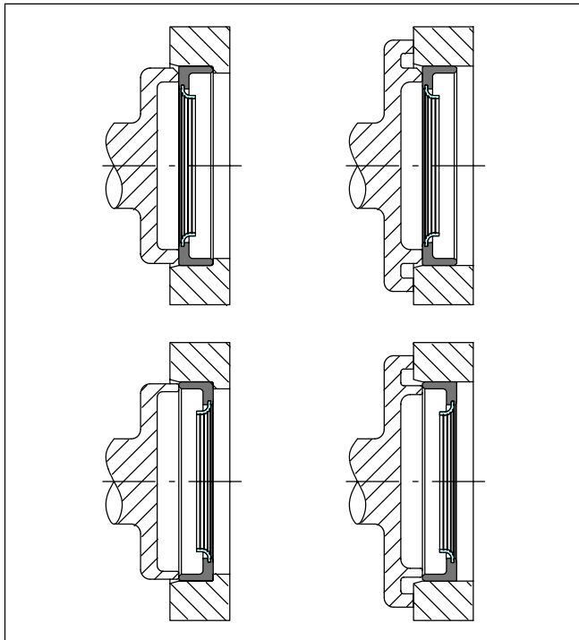
Figure 16 Assembly techniques
