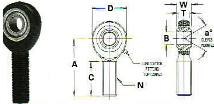
ALRSM - EXTRA STRENGTH ALUMINUM - HEAVY DUTY SHANK
