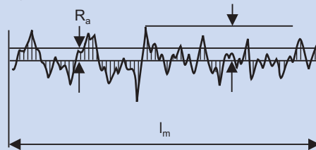
Figure 5-4: Roughness Terminology
