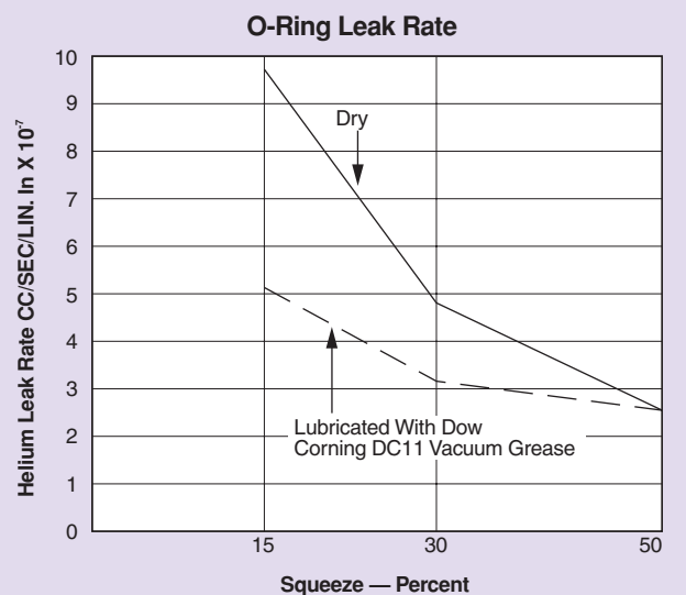
Figure 3-8: O-ring Leak Rate
