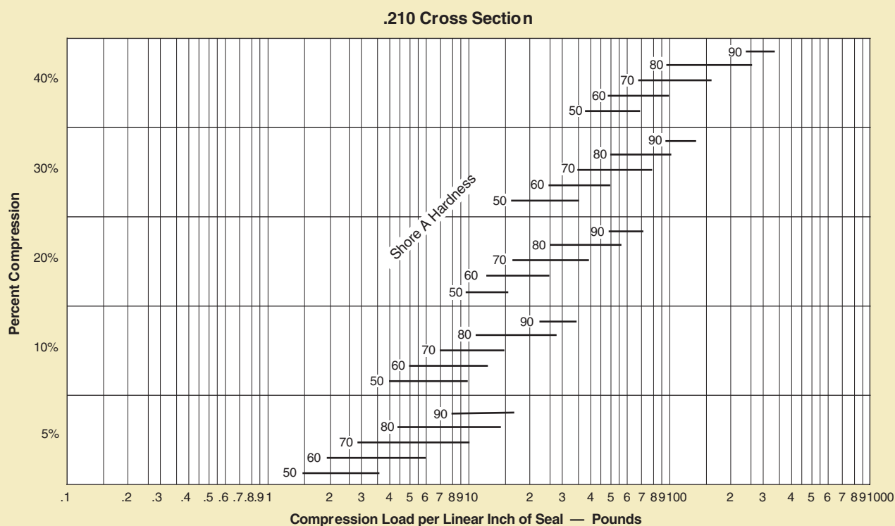
Figure 2-7: .210 Cross Section
