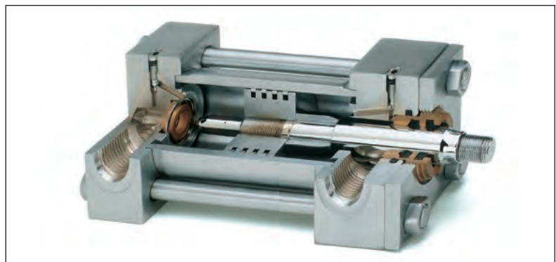
Fig. 2-1. Hydraulic cylinder
