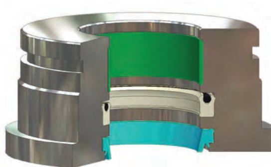
BD Installed in Rod Gland
